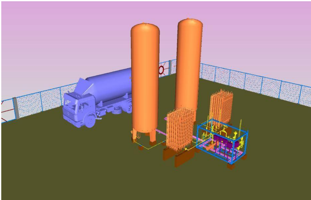
3D Modeling of LIN Storage Tank
