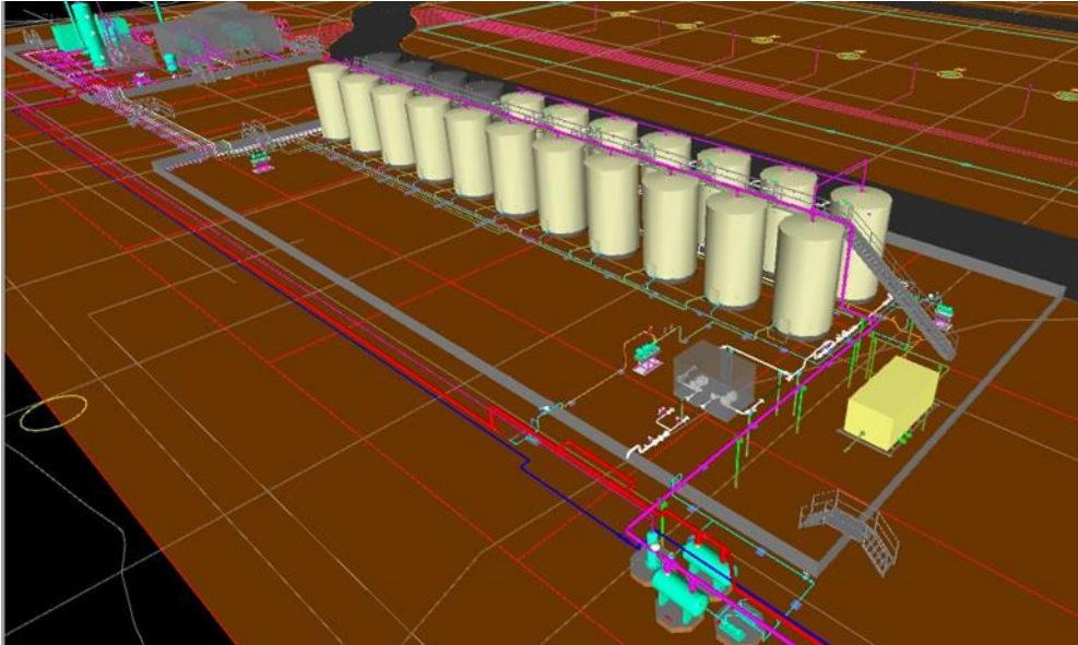
3D Modeling – Tank Containments
